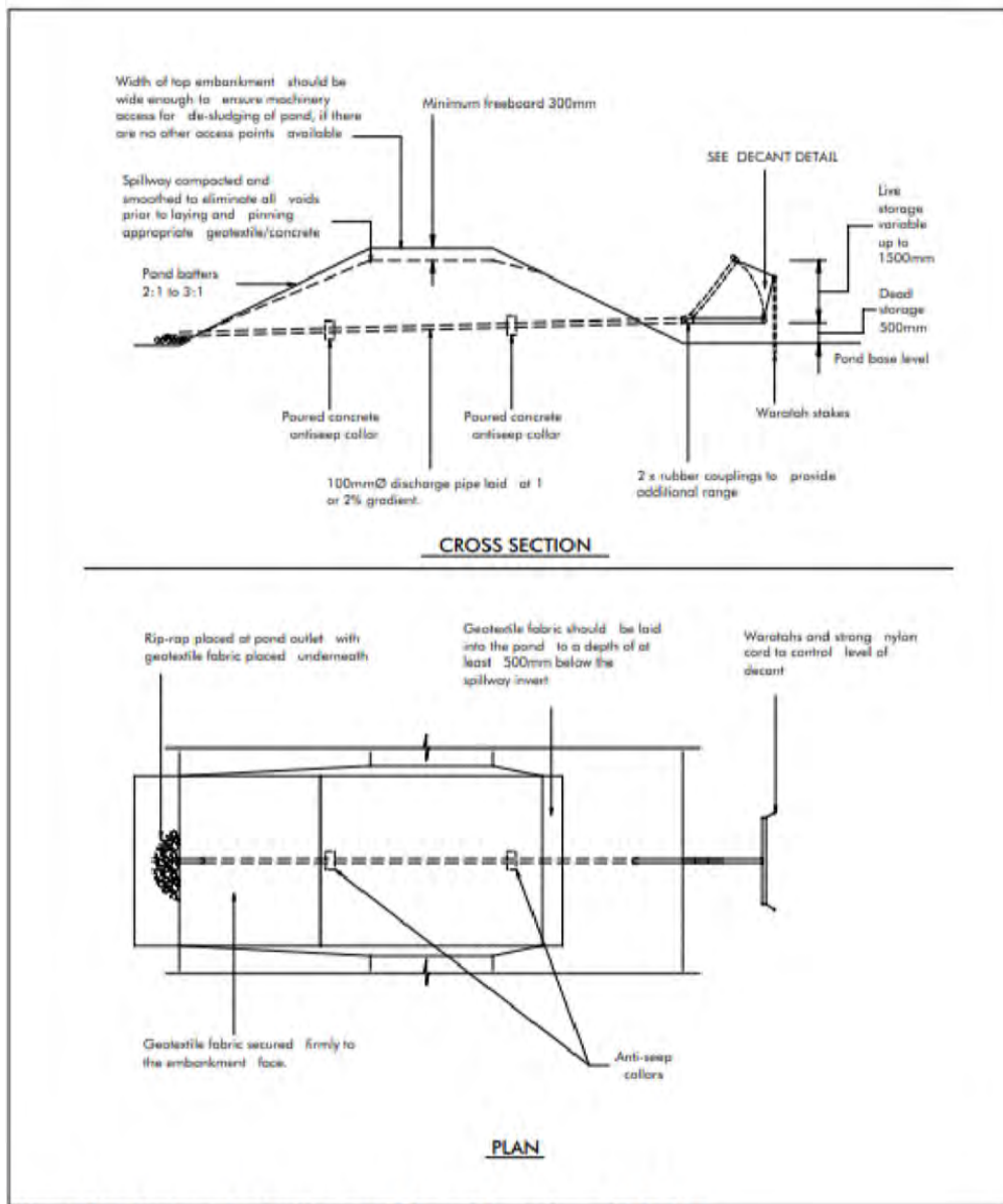
Figure 19: Sediment retention pond for catchments up to 1.5 ha
